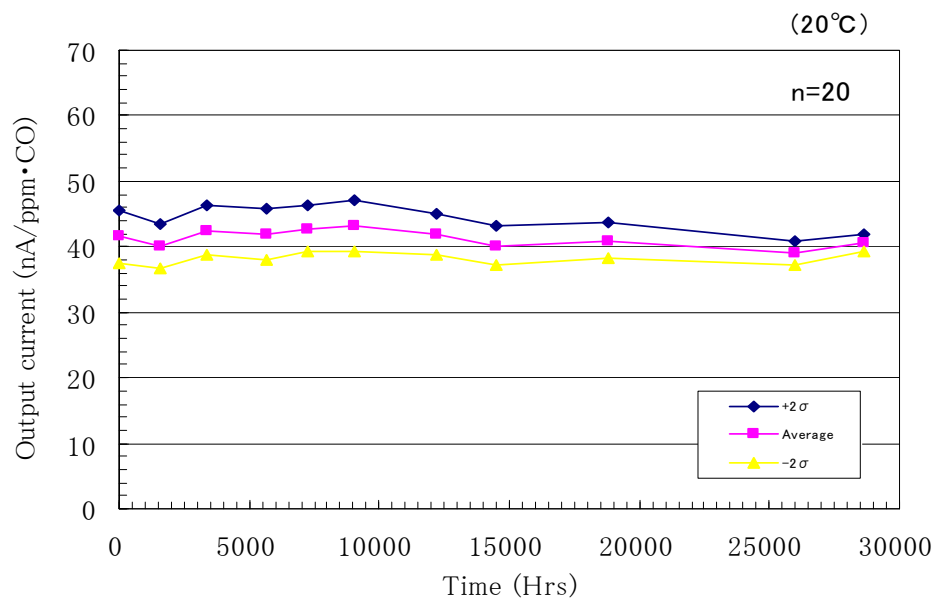
Fig. 16 Stability of sensitivity
