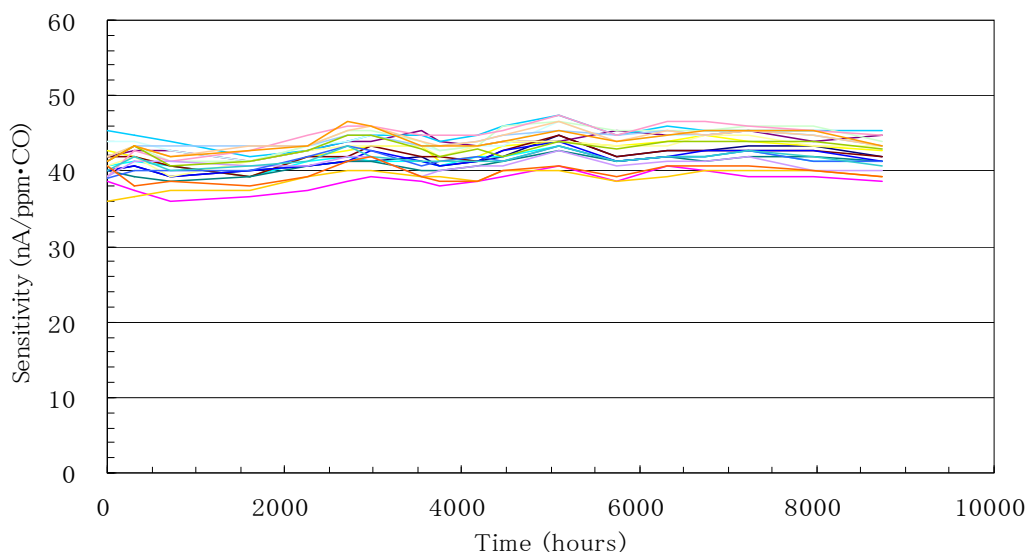
Fig. 13 Continuous exposure test in 15ppm of CO for 1 year
