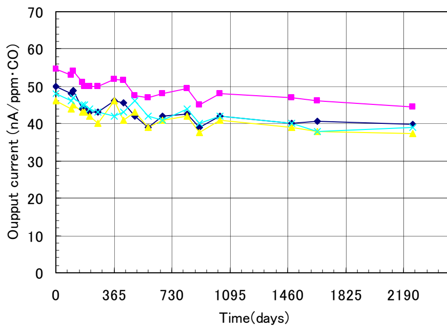
Fig.3 Long term stability of sensor developed in 2000 (Reference data)
