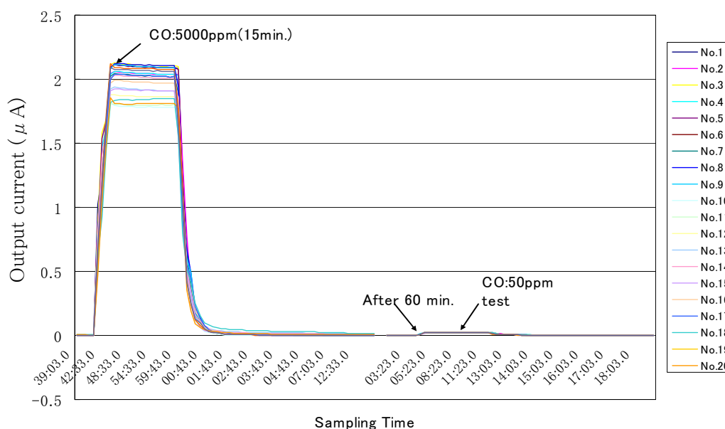
Fig.14 Exposure test in 5000ppm of CO for 15min. (EN50291)
