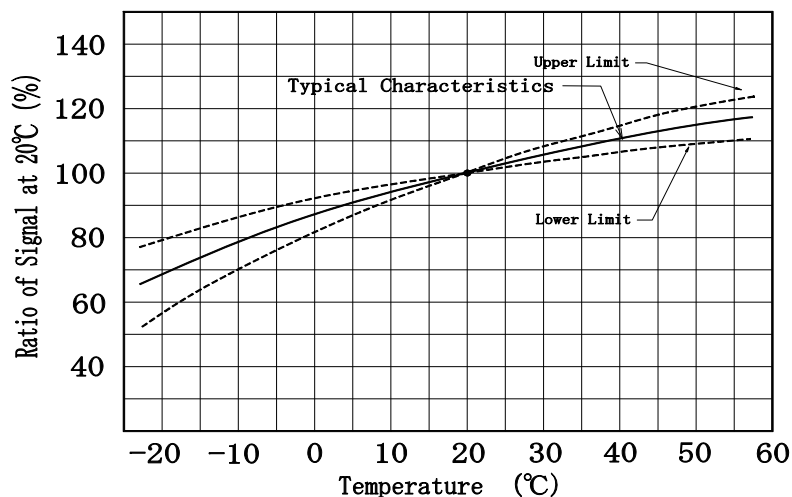
Fig. 12 Temperature dependence
