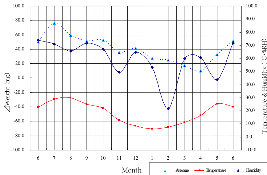
Fig. 20 Relationship between electrolyte quantity and climate variation (Outside)
