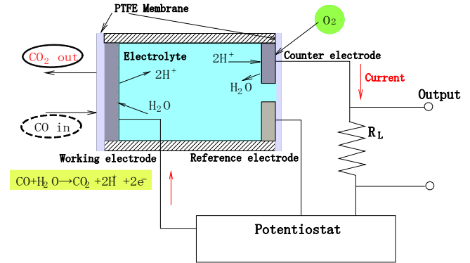
Fig.1 Detection principle
