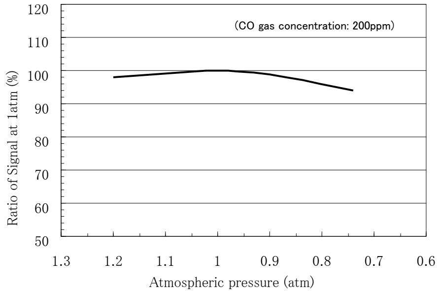
Figure 8 shows the typical data of pressure dependence on NAP-505.
